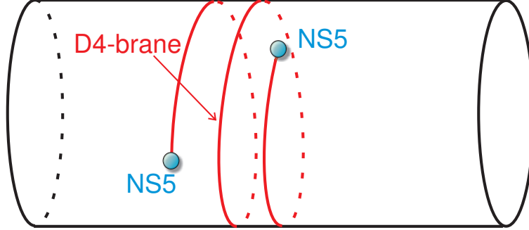
Figure 1: T-dual, “brane box”, description of this configuration, in which the fractional D3-brane becomes a D4-brane stretched between two NS5-branes on a T-dual circle. Moving in the b direction through multiple periods in closed string moduli space in the original description corresponds to moving one of the NS5-branes around the circle, dragging the D4-brane around with it so as to introduce multiple wrappings.
