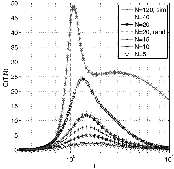
Fig. 2 Divergence of the heat capacity is a classical signature of criticality. This plot represents the heat capacity versus temperature for Ising models of retinal activity for increasing population sizes N [82]. The “ N = 20 , rand,” and N = 120 curves were obtained by inferring Ising models for fictitious networks whose correlations were randomly drawn from real data. Error bars show the standard deviation when choosing different subsets of N neurons among the 40 available
